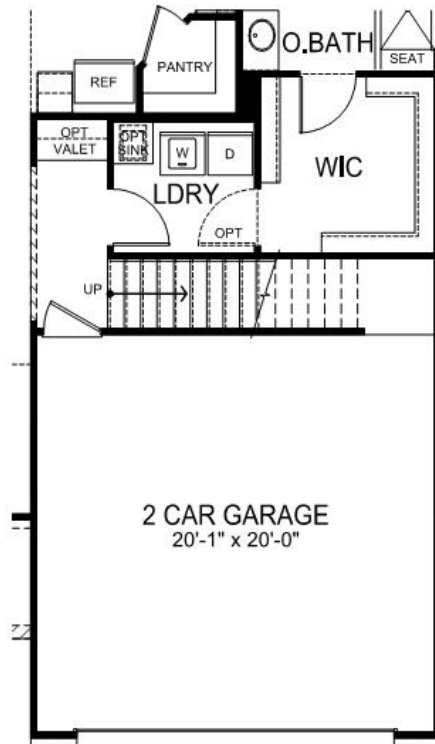
STAIRS AND OPT 2ND FLOOR
