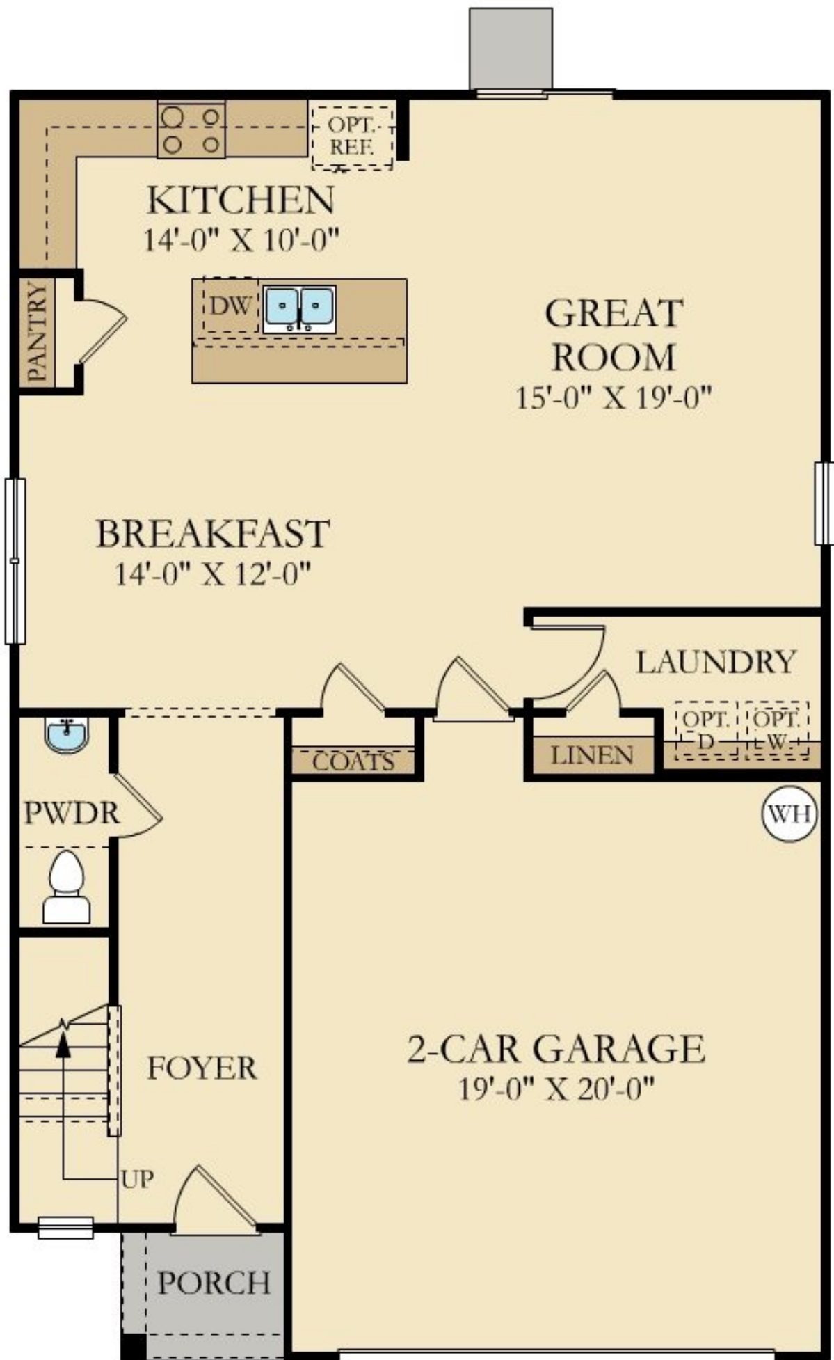
FIRST FLOOR
