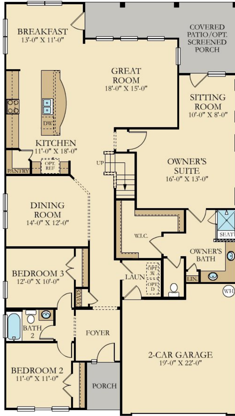
FIRST FLOOR
