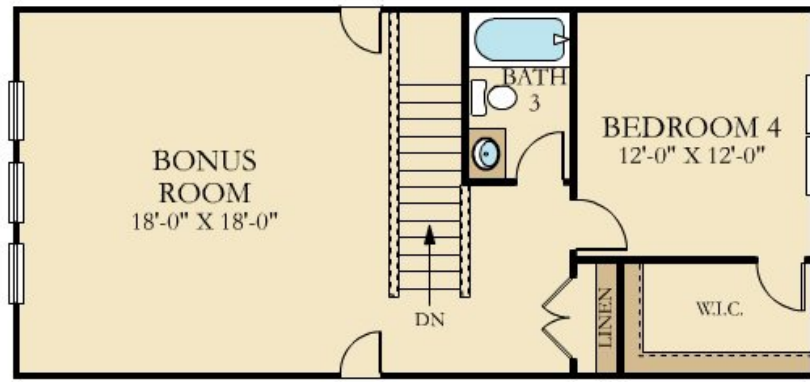
SECOND FLOOR
