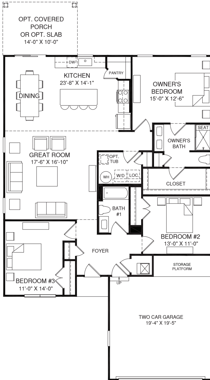
MAIN LEVEL
