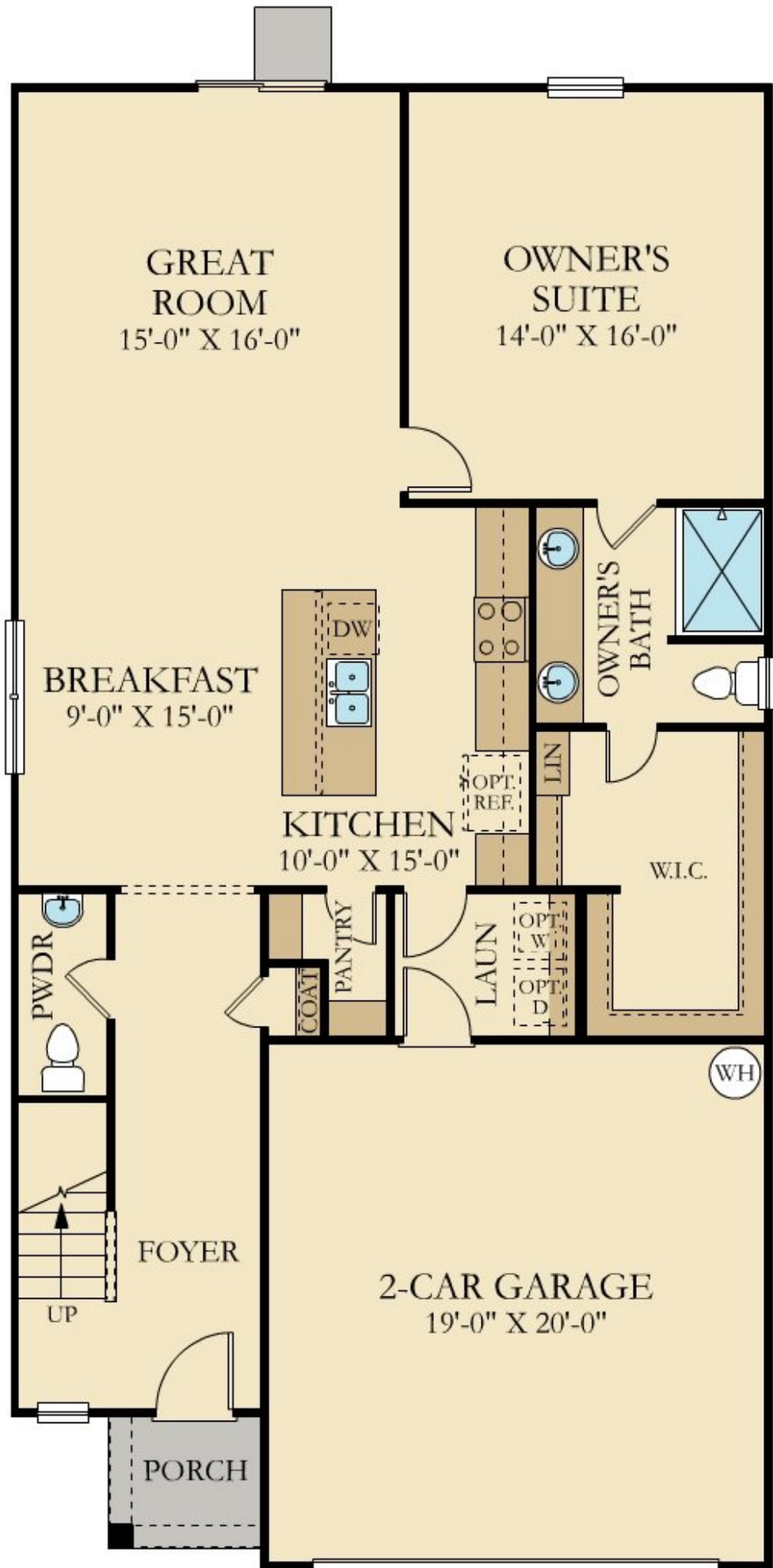
FIRST FLOOR
