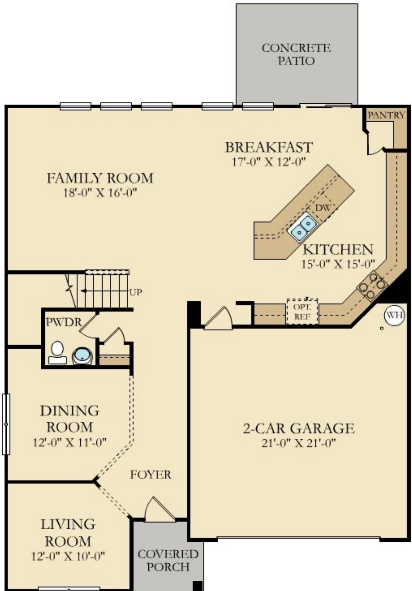
FIRST FLOOR
