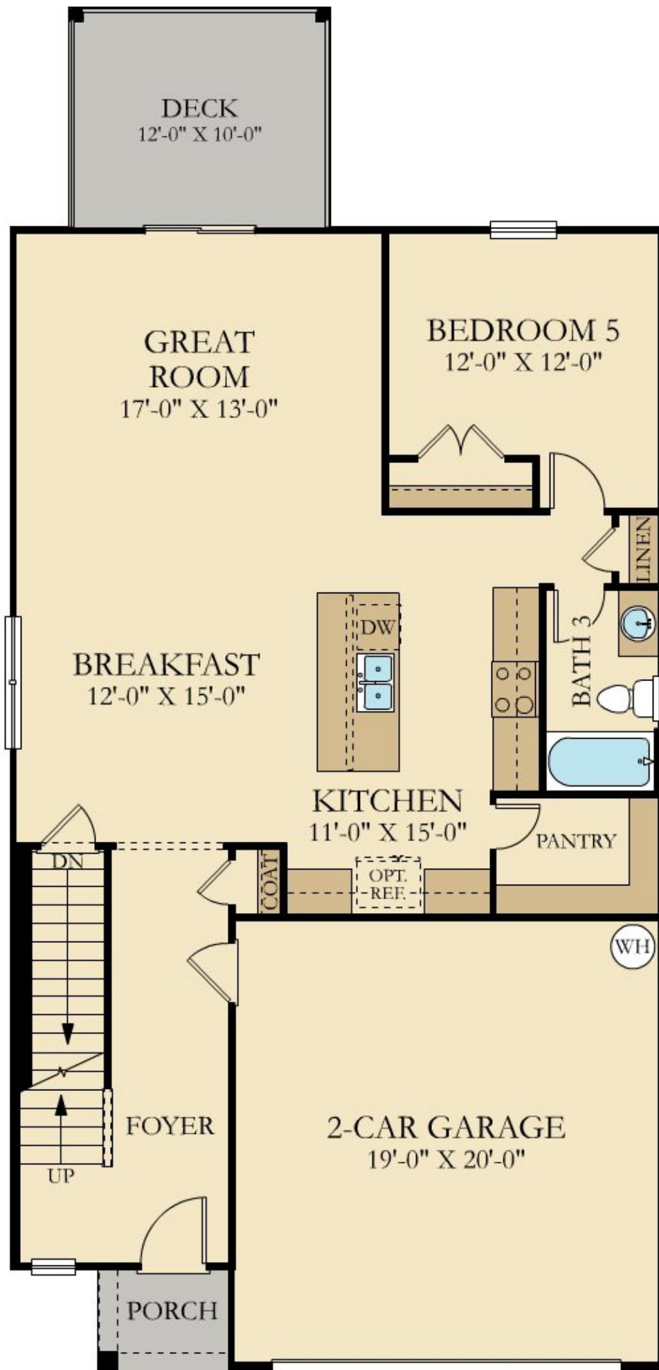
FIRST FLOOR
