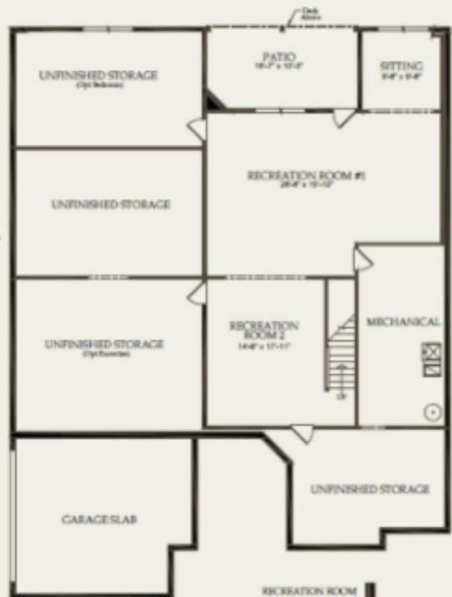
Finished Basement
