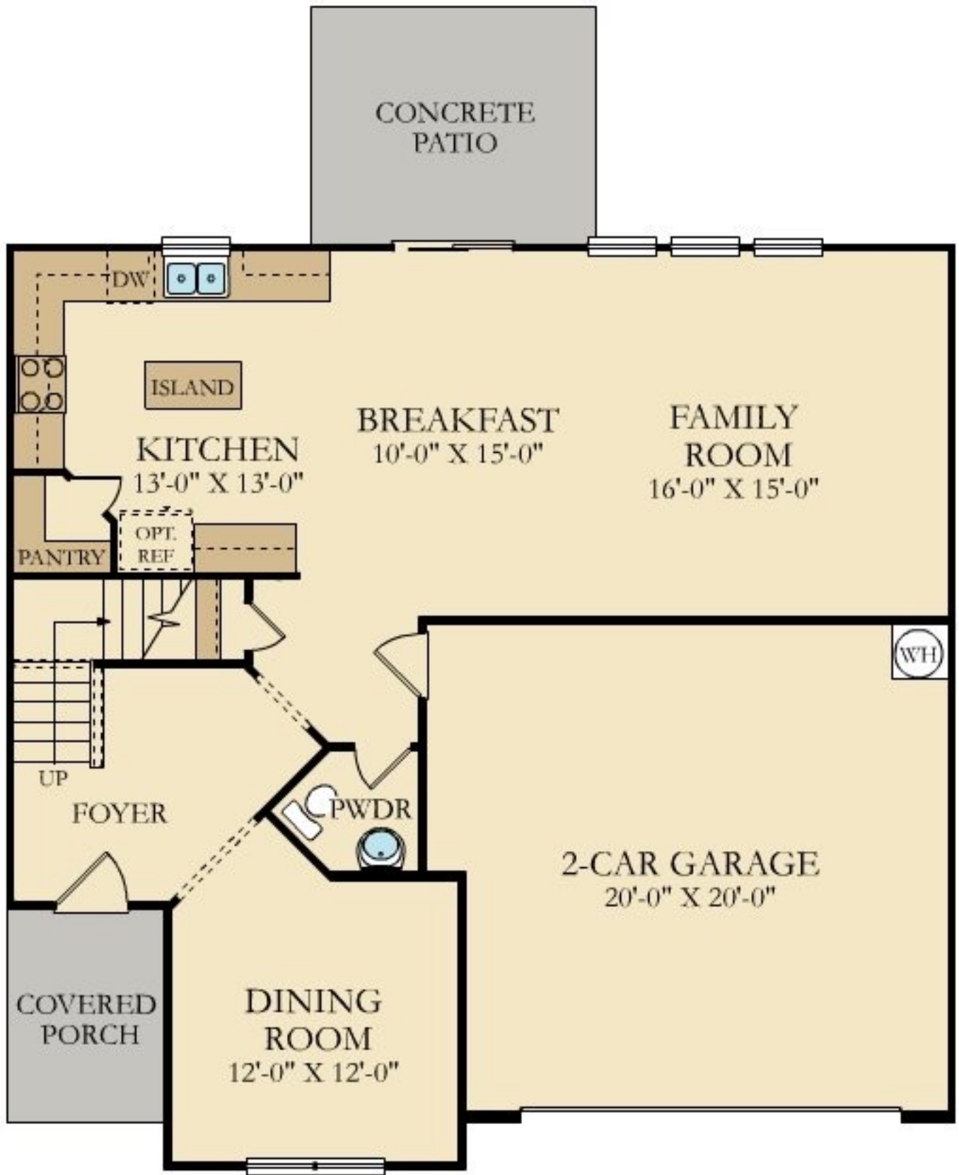
FIRST FLOOR
