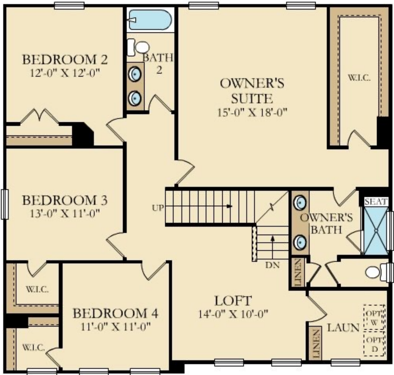
SECOND FLOOR
