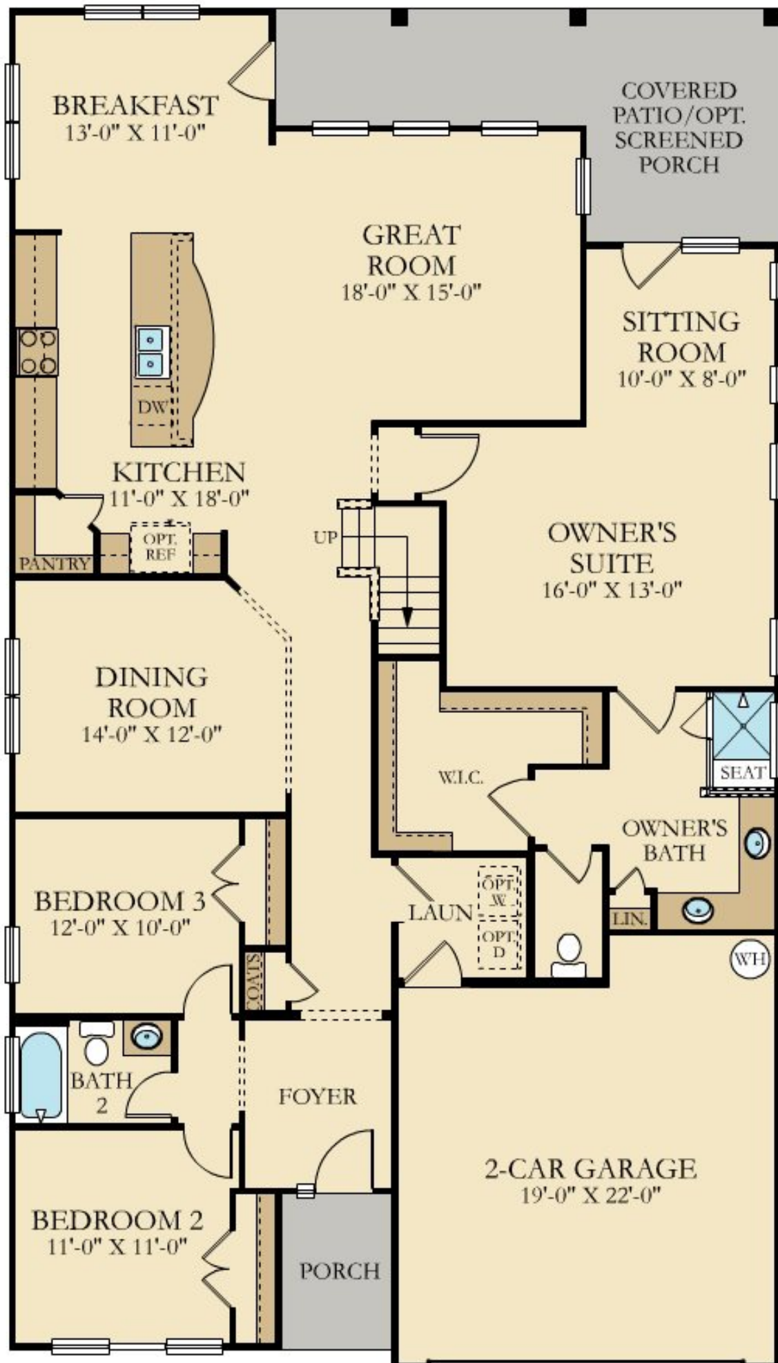
FIRST FLOOR
