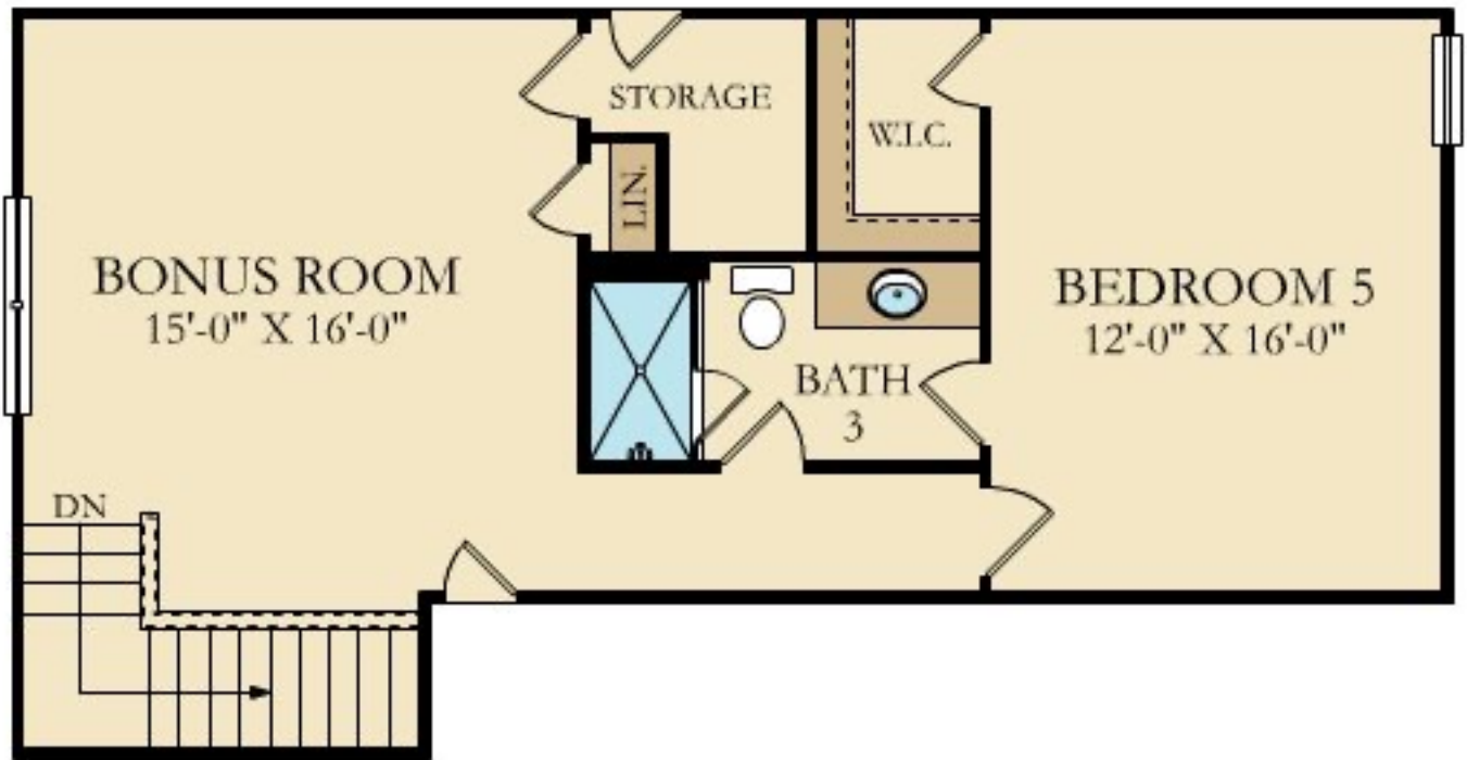
THIRD FLOOR
