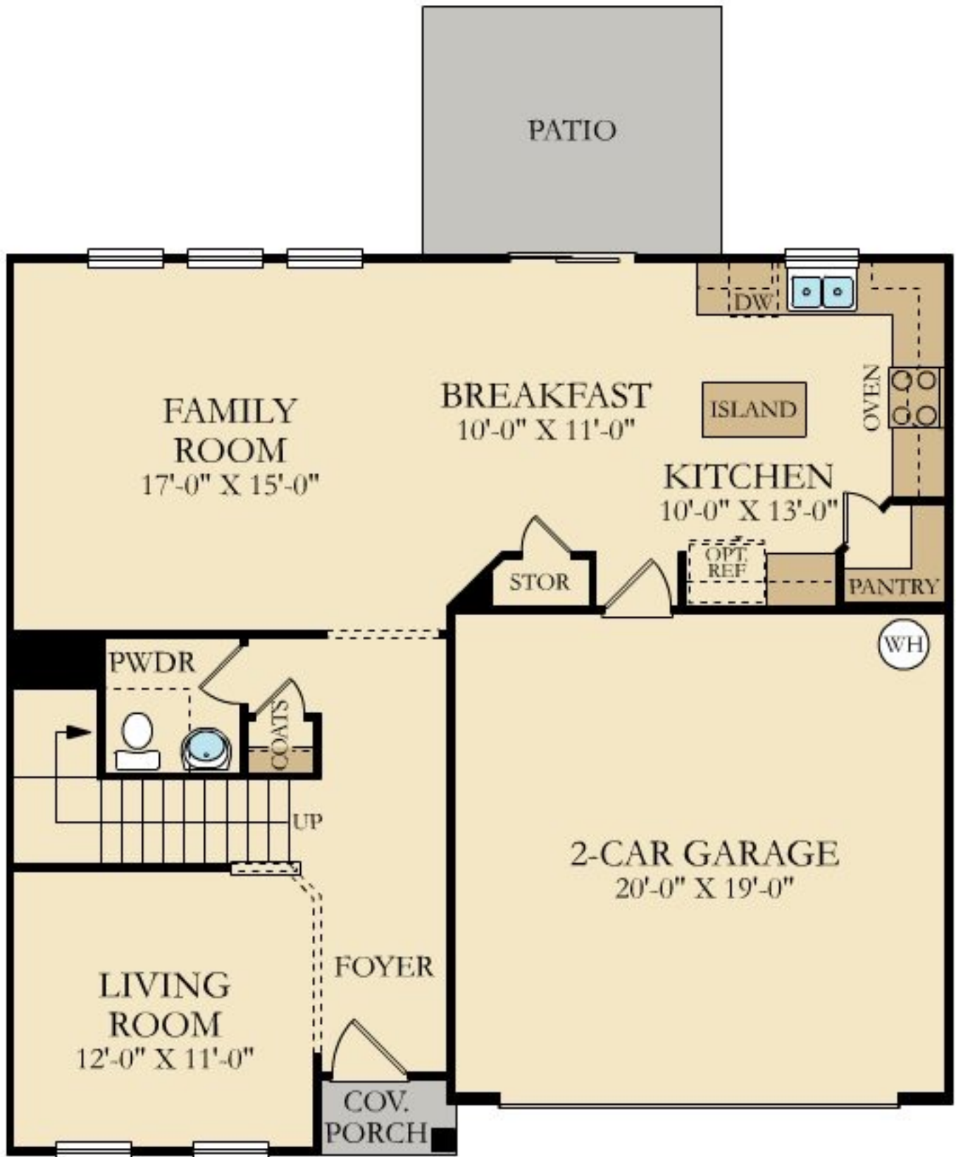
FIRST FLOOR
