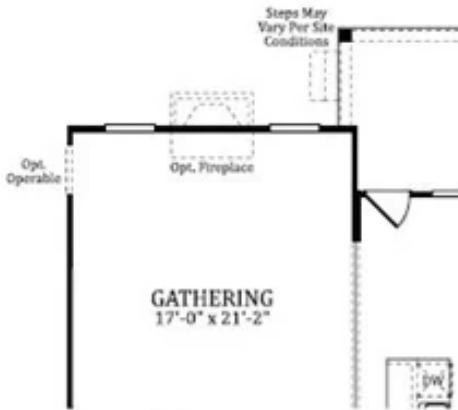
OPT. 4' GATHERING EXTENSION
