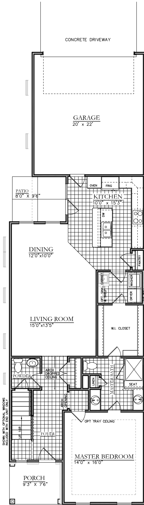
1ST FLOOR
