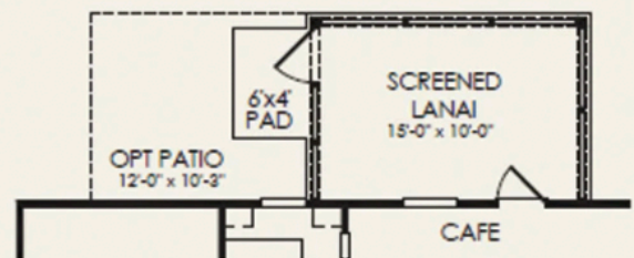
Opt Screened Lanai
