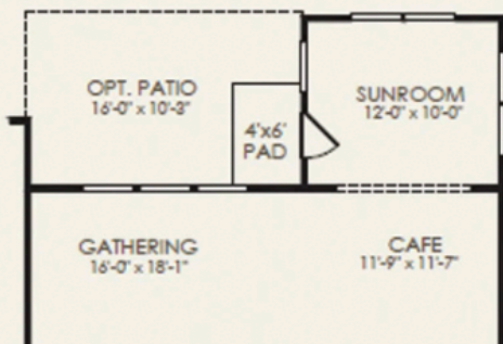
Opt. Sunroom
